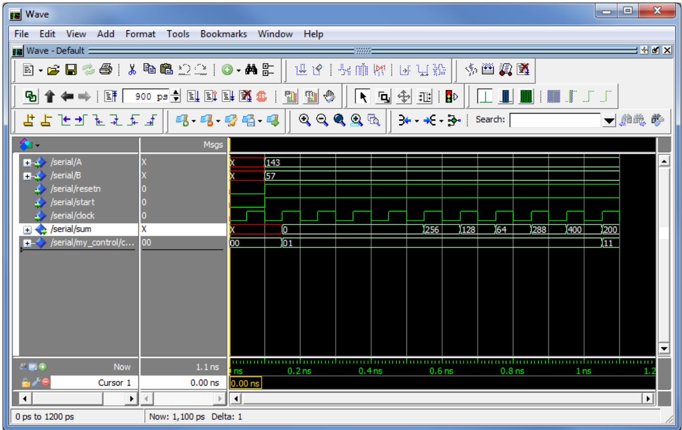
Figure 20. Simulation results after 1100 ps.
