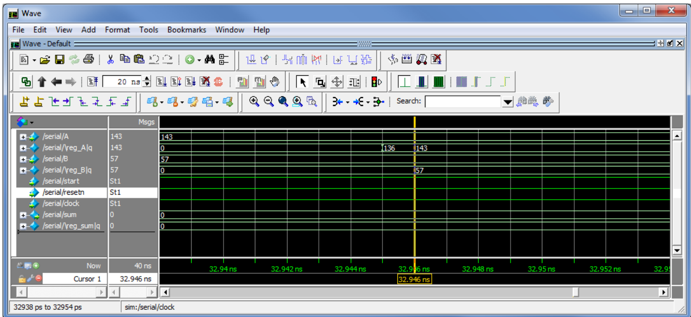
Figure 27. Zoomed-in Timing Simulation after 40ns.
