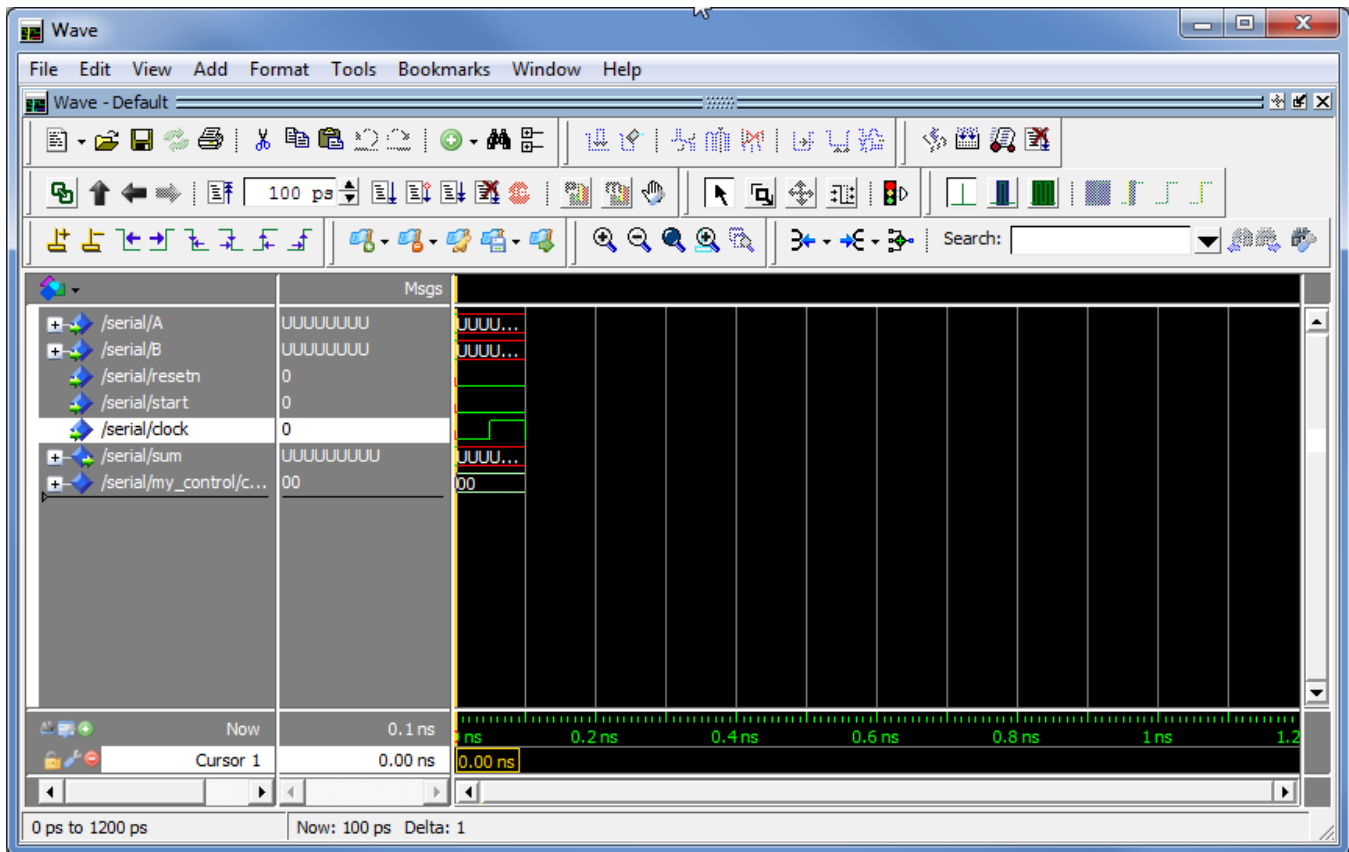
Figure 17. Simulation results after 100 ps.
