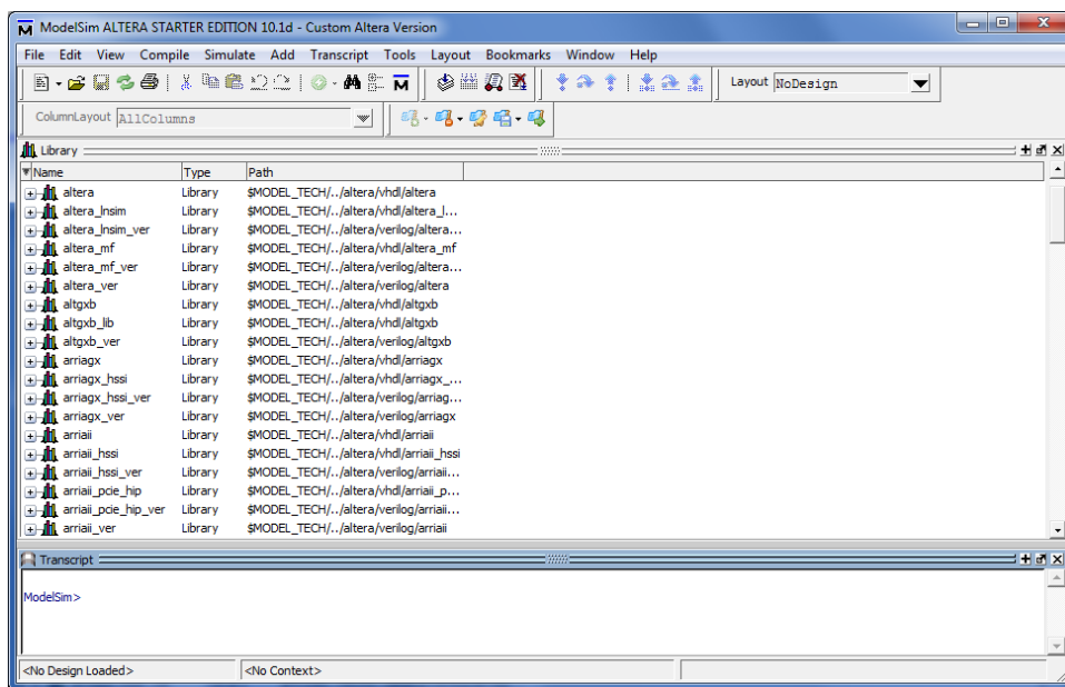
Figure 7. ModelSim window.
